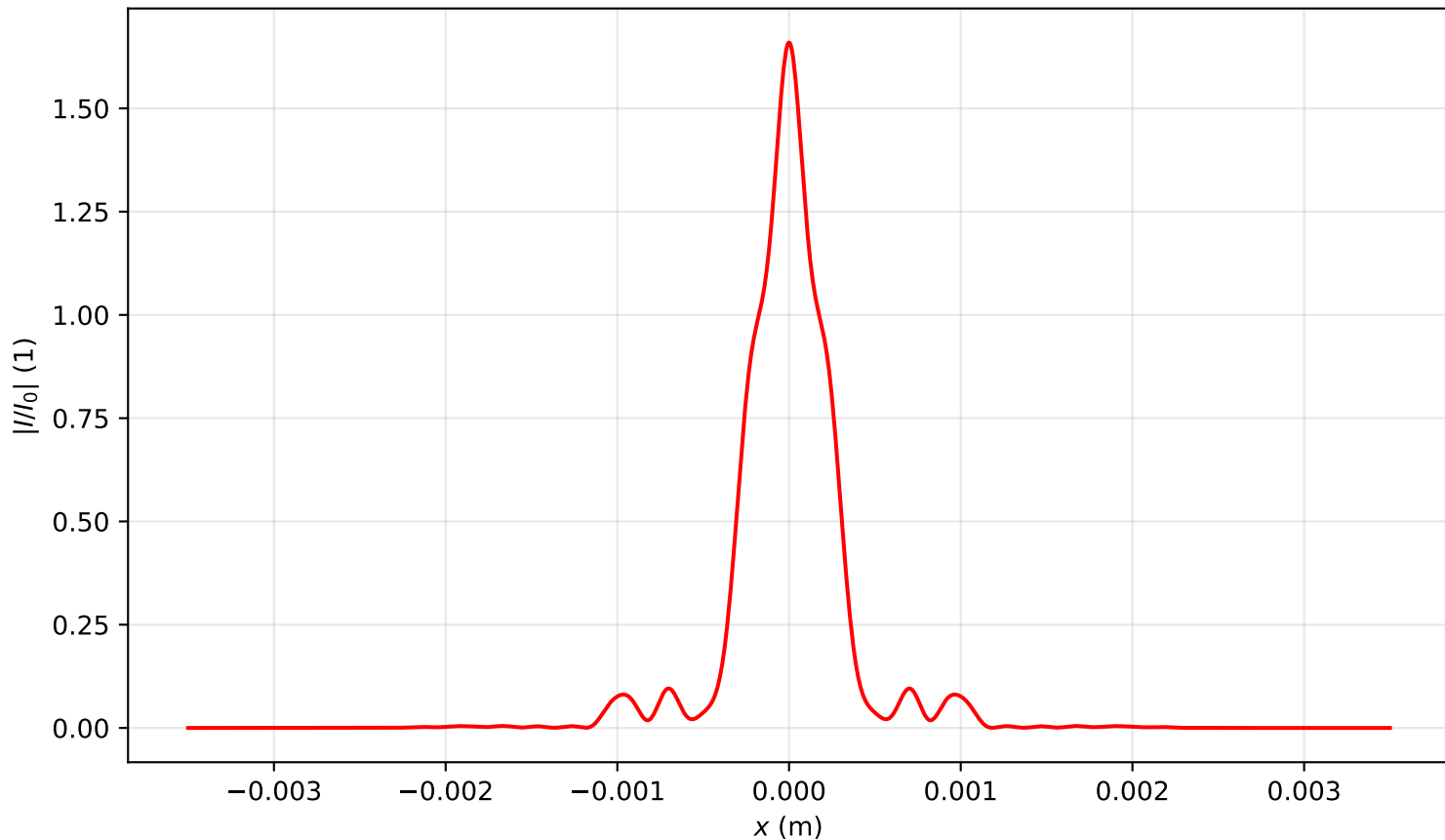
Intensity profile I(x, y = 0, z = 1.194)/I_0 , P_{in}=6.5P_{cr} , artificial time
